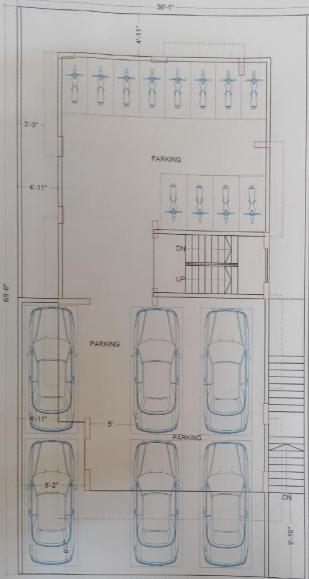
PARKING FLOOR PLAN
