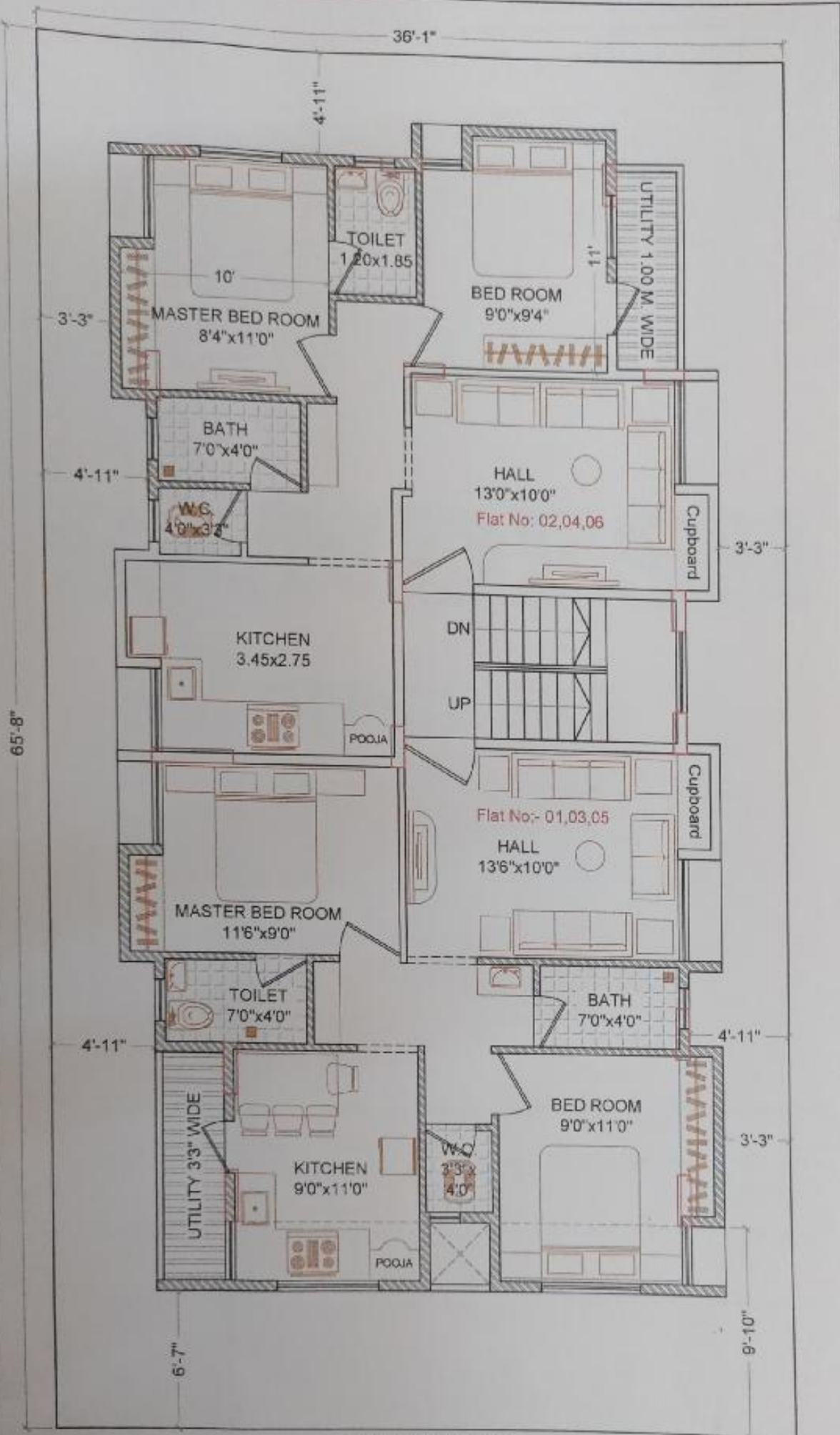
TYPICAL FIRST+SECOND & THIRD FLOOR PLAN
